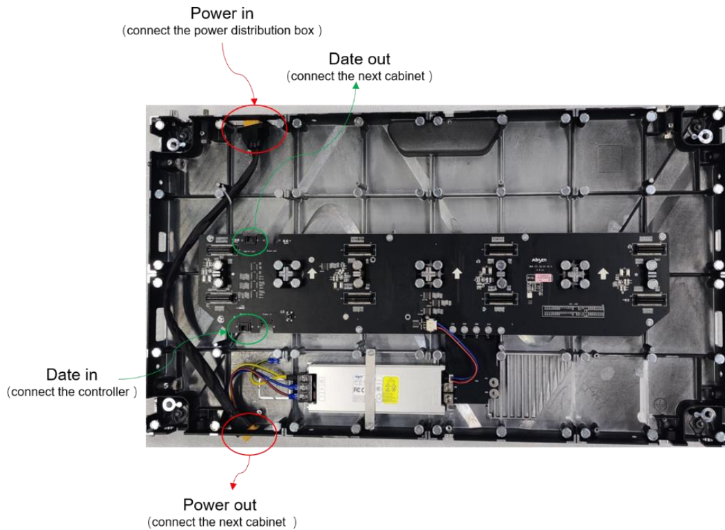
Power and signal connections inside the cabinet
