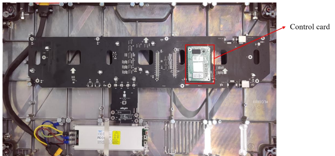
Power and signal connections inside the cabinet
